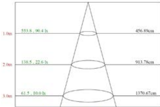
Max., Ave Beam angle of C10 plane 132.72
